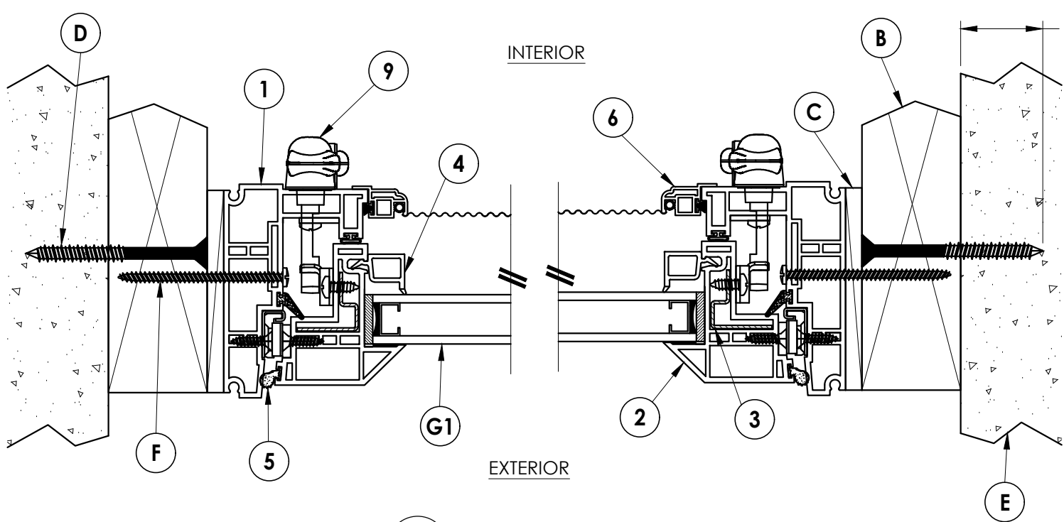
1 HORIZONTAL CROSS SECTION 2 2X Buck Construction
