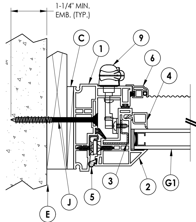
3 HORIZONTAL CROSS SECTION 3 Shown w/ TX sub-buck
