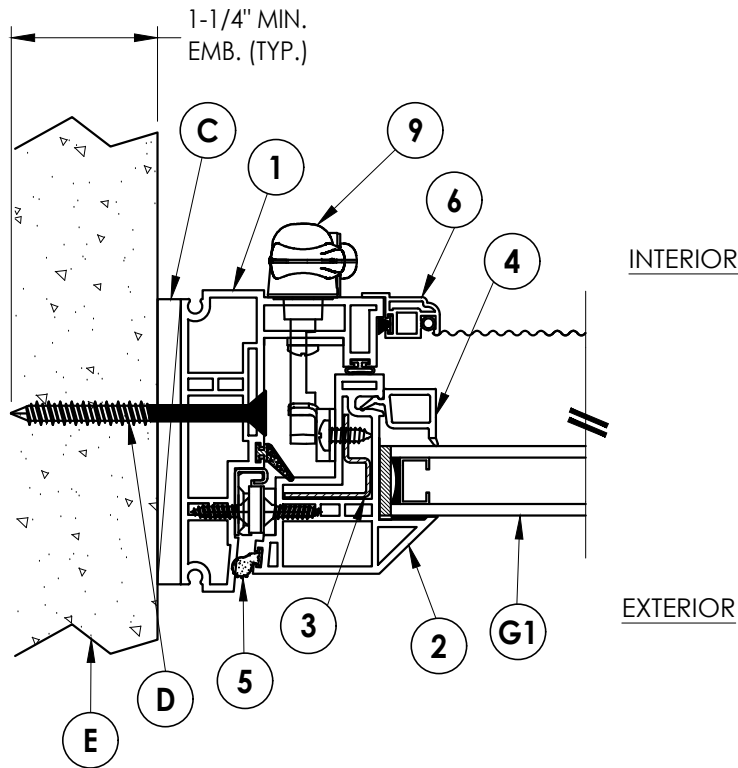
1 HORIZONTAL CROSS SECTION 3 Shown Direct to Masonry
