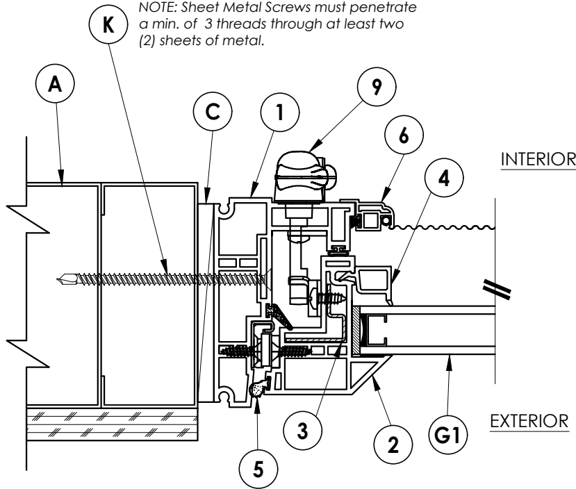
2 HORIZONTAL CROSS SECTION 3 Shown w/ Steel Stud Framing Option
