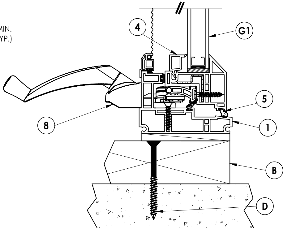
2 VERTICAL CROSS SECTION 2 2X Buck Construction
