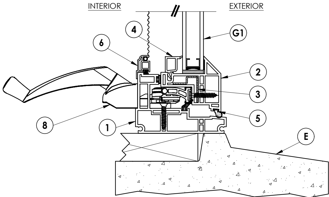
4 VERTICAL CROSS SECTION 3 Optional masonry sill
